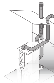
Direct-Vent Vertical
