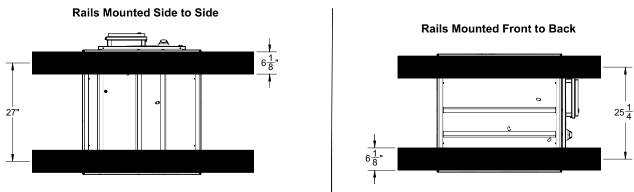
Figure 6: MHP0270R Mounting Rails Positions and Widths
