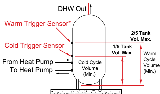
Figure 10: Multi-pass, Single Tank Sensor Locations
