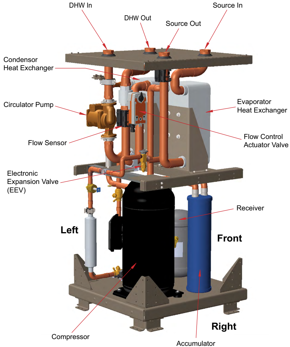
Figure 2: MHP0270R Model
