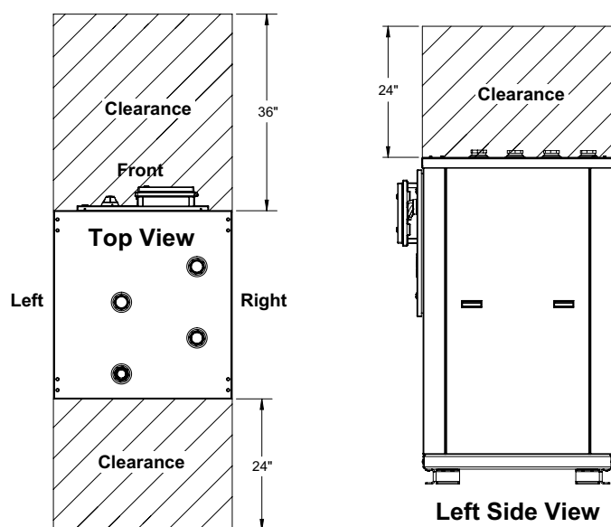
Figure 1: MHP0270R Model Clearances
