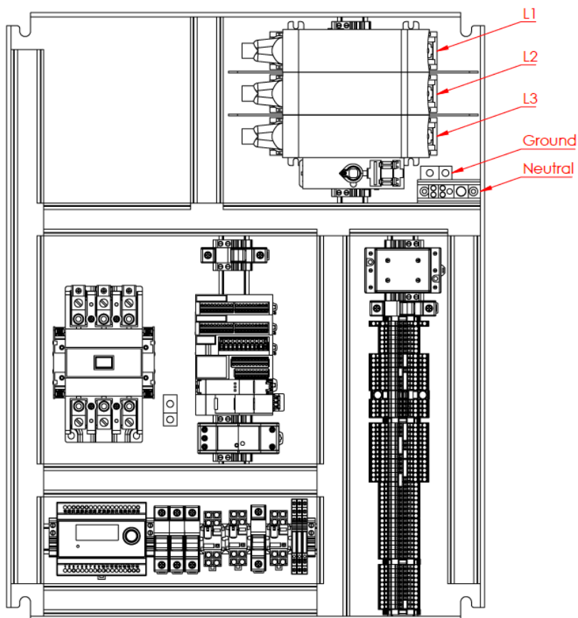
Diagram 6: Power Wiring Blackboard Orientation
