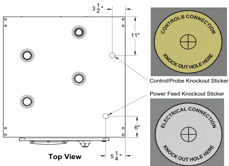
Figure 7: Wiring Knockout Locations
