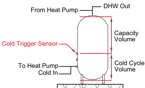
Figure 8: Single-pass Tank Sensor Location
