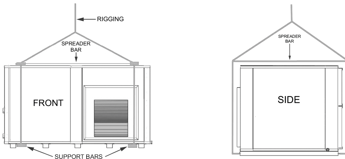
Figure 3: Rigging and Hoisting Unit
