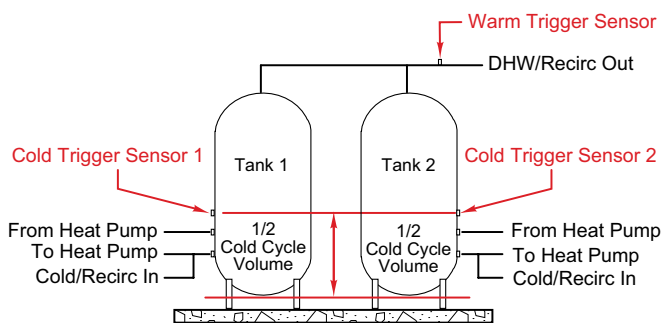
Figure 11: Multi-pass, Multiple Tanks with Central Controller
