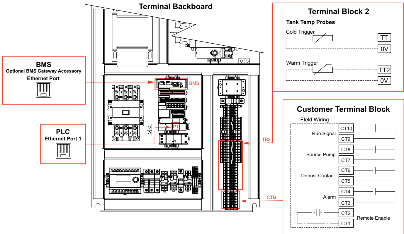
Diagram 8: MHP0270R Field Wiring Control Points
