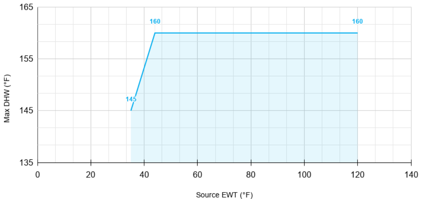
Diagram 1: MHP0270R Source EWT – Maximum DHW LWT for Single-Pass Operation
