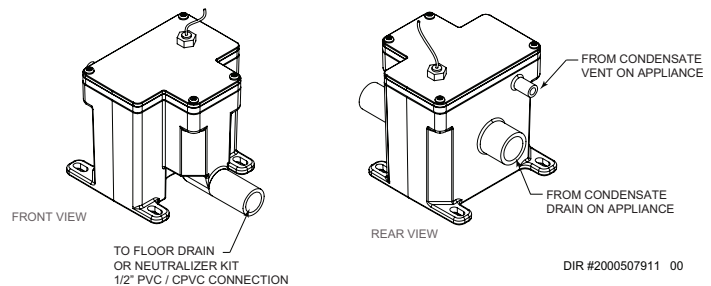
Figure 2-1 Condensate Trap
