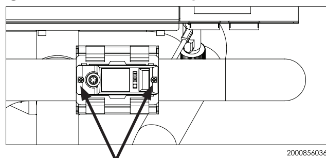
Figure 2-6 Removal of mounting screws
