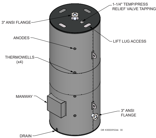
Figure 5-2_Vertical Storage Tank w/Anodes
