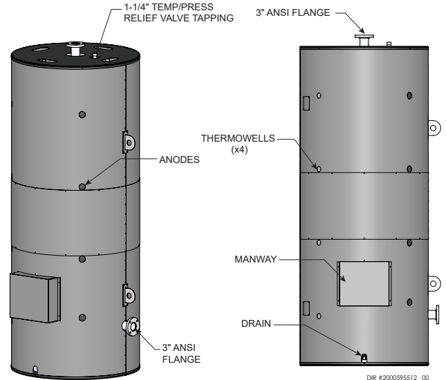
Figure 5-1_Vertical Tank
