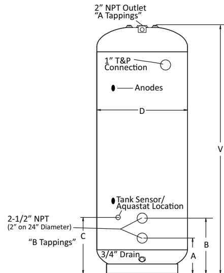
24" & 28" DIAMETER TANKS
