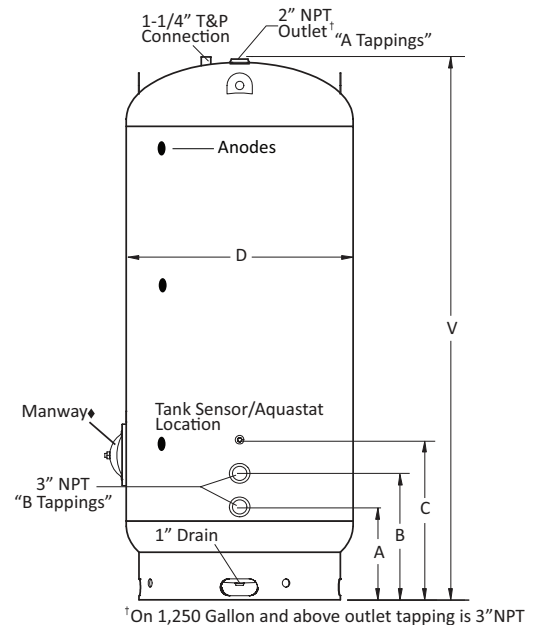
30" DIAMETER AND LARGER TANKS
