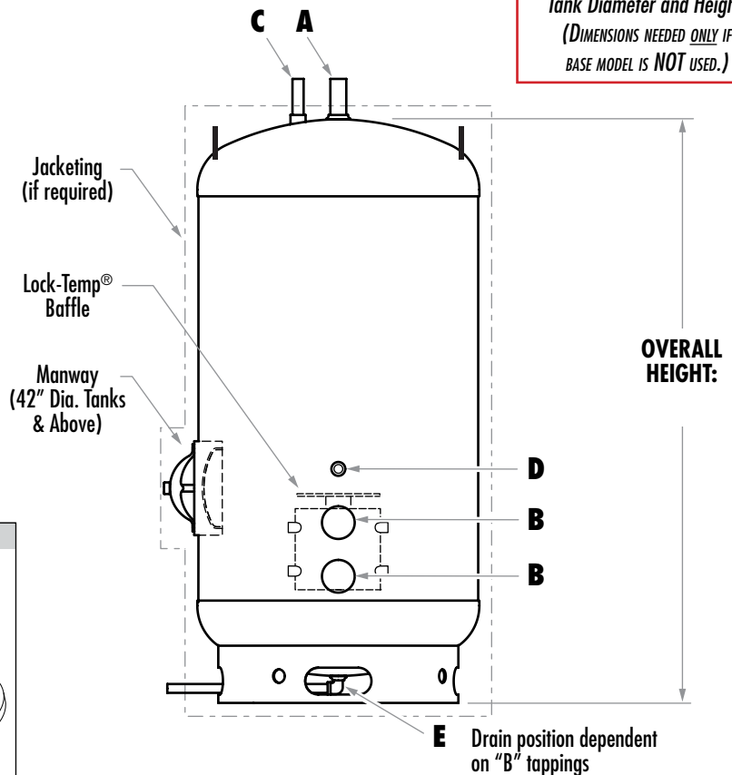
NPT - Threaded
