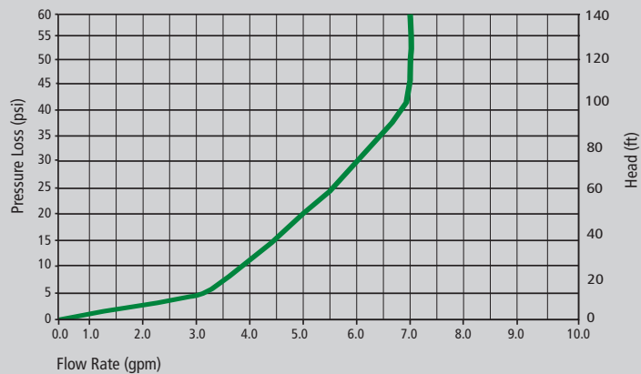
140H: Pressure Loss
