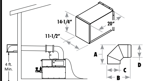
VENT ADAPTER
