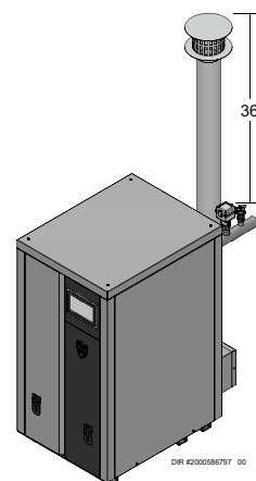
Figure 6-1 Installation extérieure
