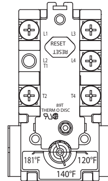
Figure 4. A-8 Thermodisc Thermostat
